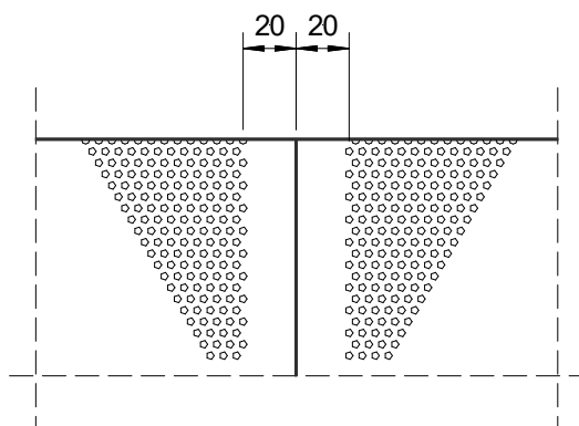
Lochblech Rv 3 - 5
